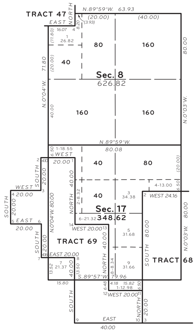
Figure 9-11. Normal tract segregations, with lotting of the adjoining Federal interest land. The tract segregations are laid out on the plat as any private land claim would be shown on an original plat.
